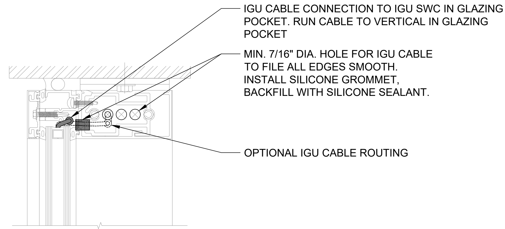
DETAIL 1 HEAD
