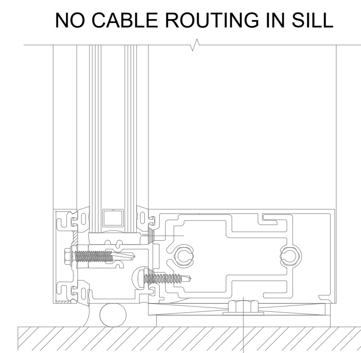
DETAIL 3 SILL
