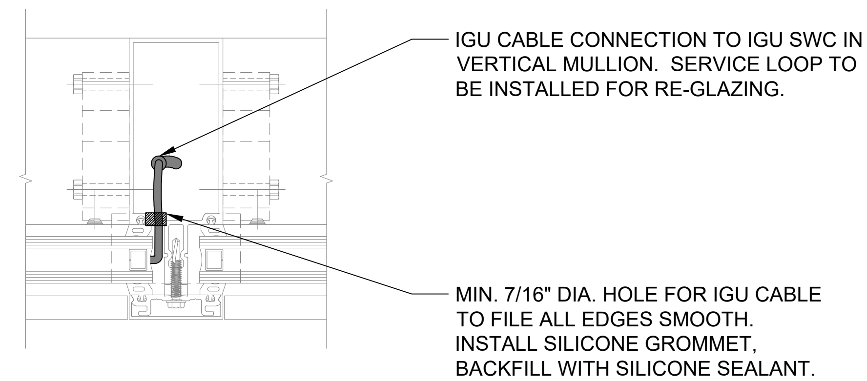
DETAIL 5 VERTICAL MULLION
